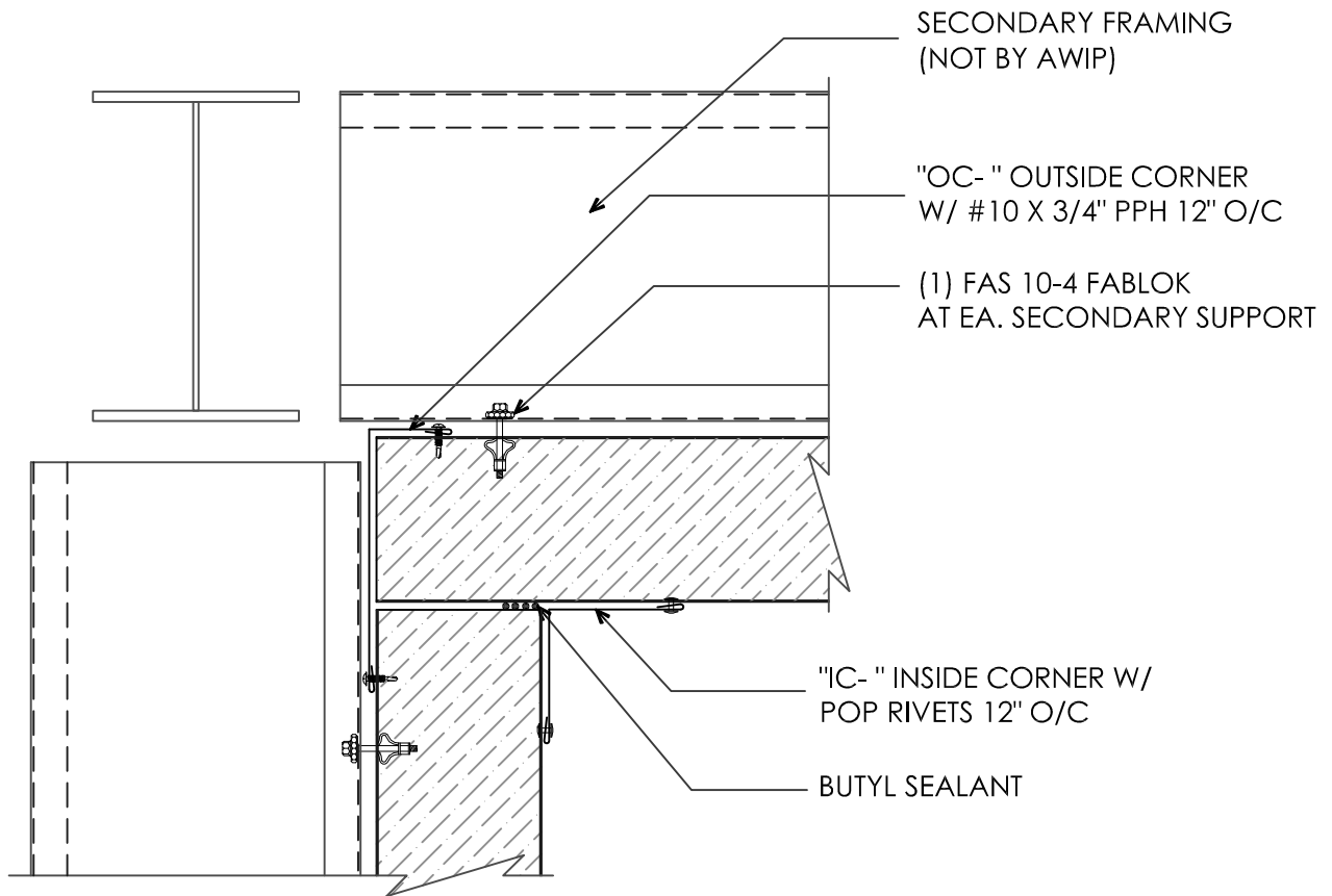
INSIDE CORNER (PLAN VIEW)
