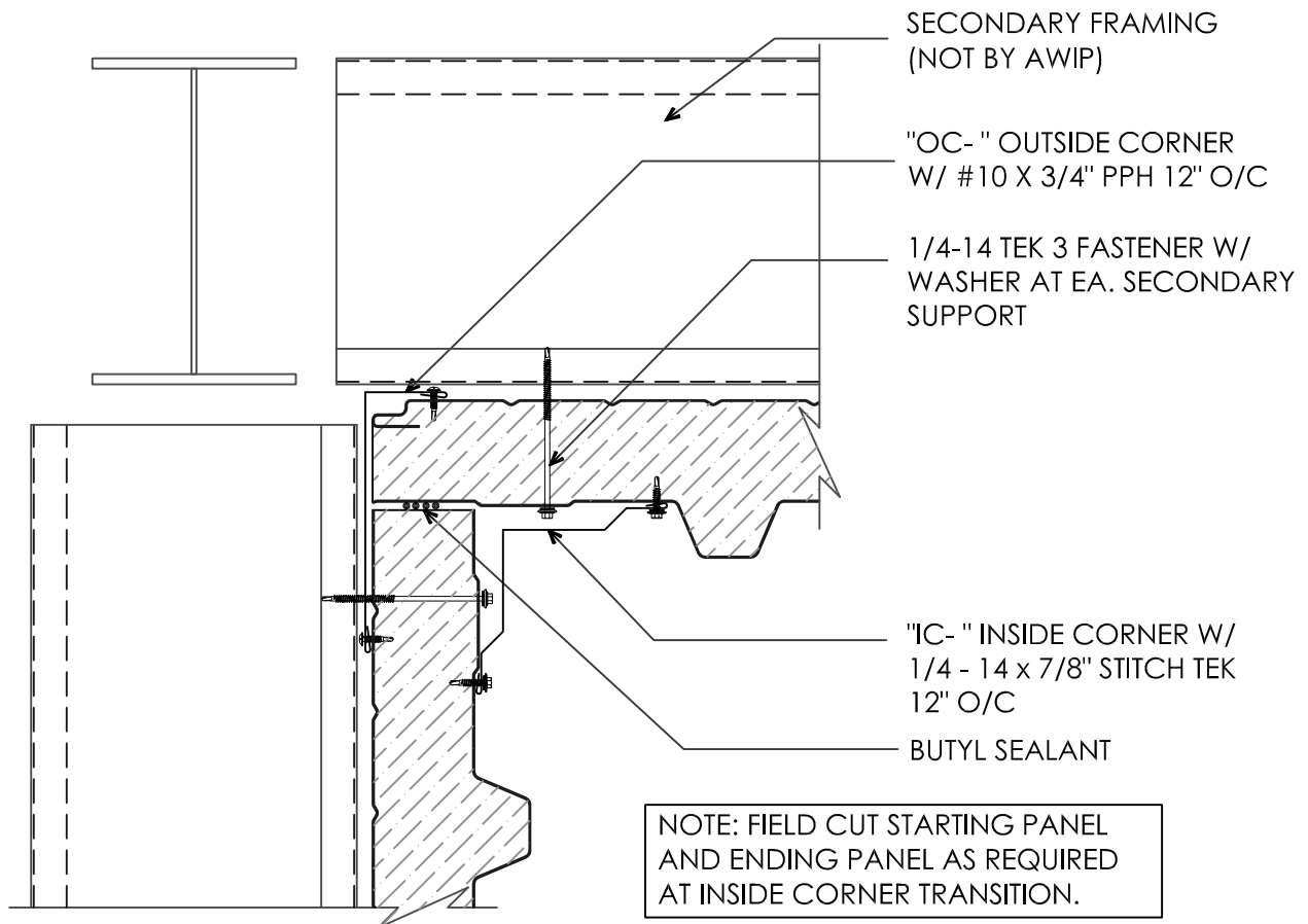
INSIDE CORNER (PLAN VIEW)
