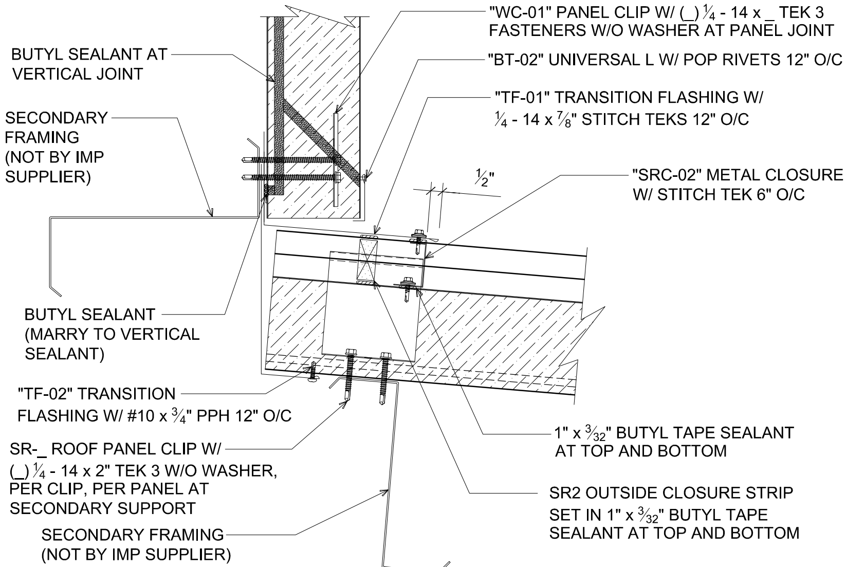
# HIGH EAVE SIDE WALL TO ROOF (SECTION VIEW)
