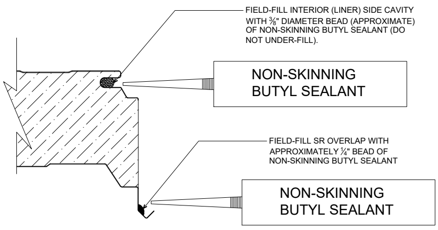
SEALANT PLACEMENT AT PANEL JOINT
