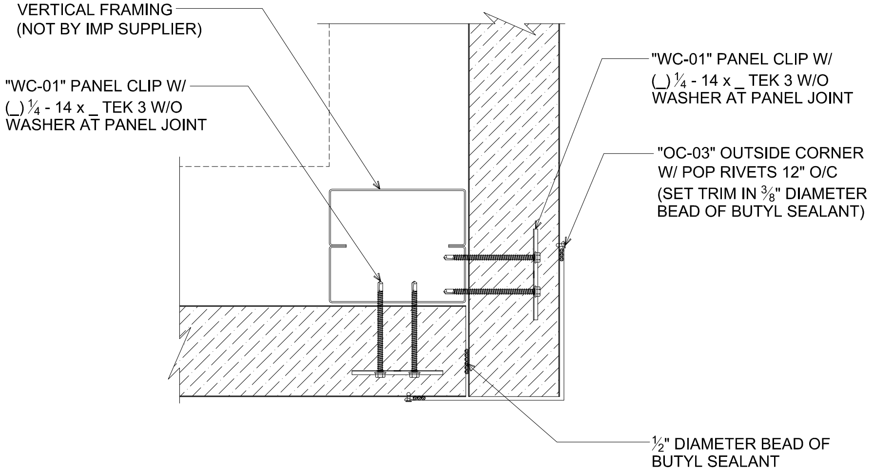
# CORNER TRANSITION - FLAT OUTSIDE (PLAN VIEW)
