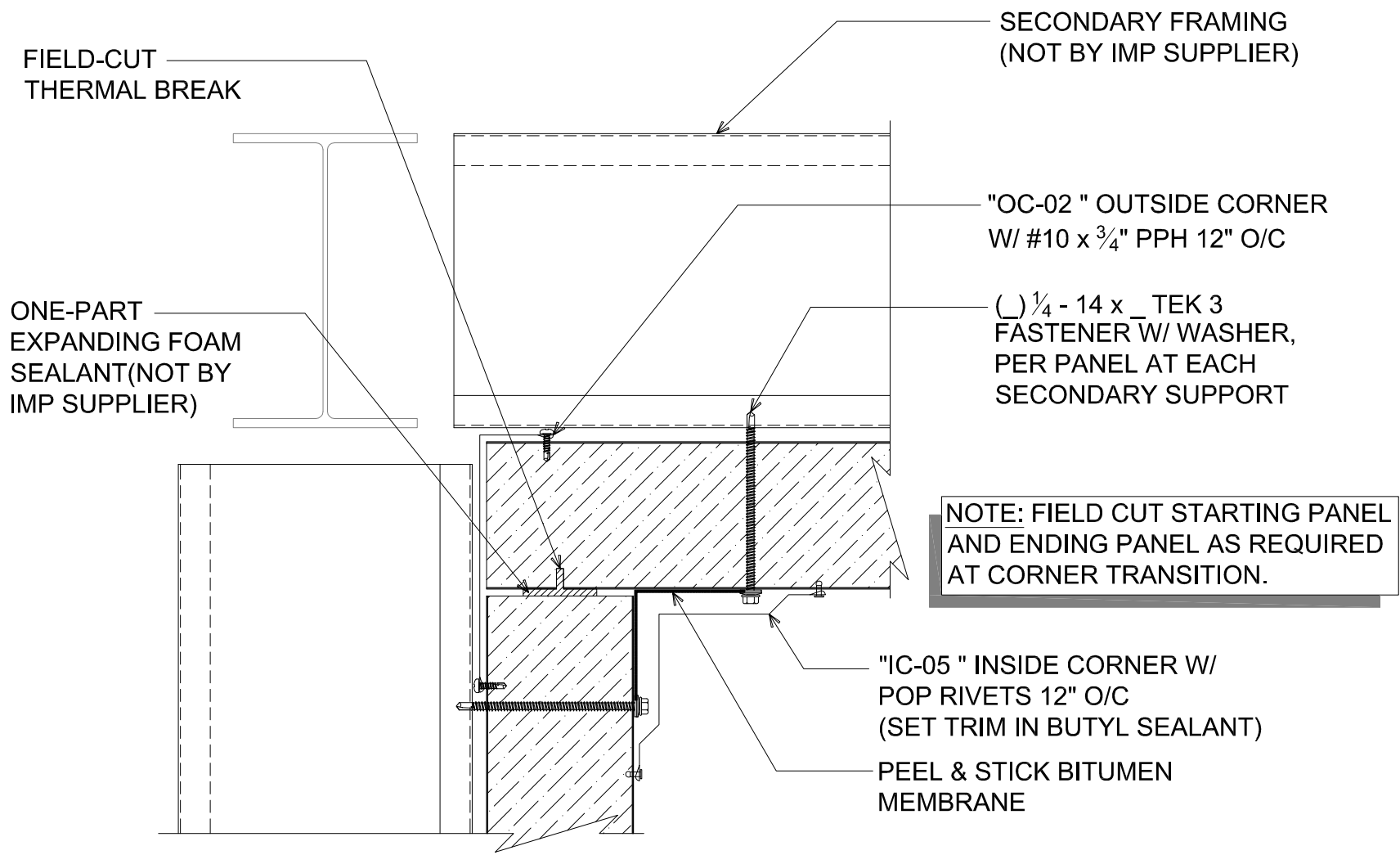
# SCULPTED INSIDE CORNER (FREEZER) (PLAN VIEW)
