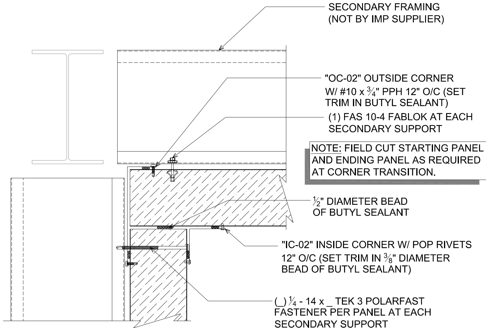
# CORNER TRANSITION - FLAT INSIDE (PLAN VIEW)
