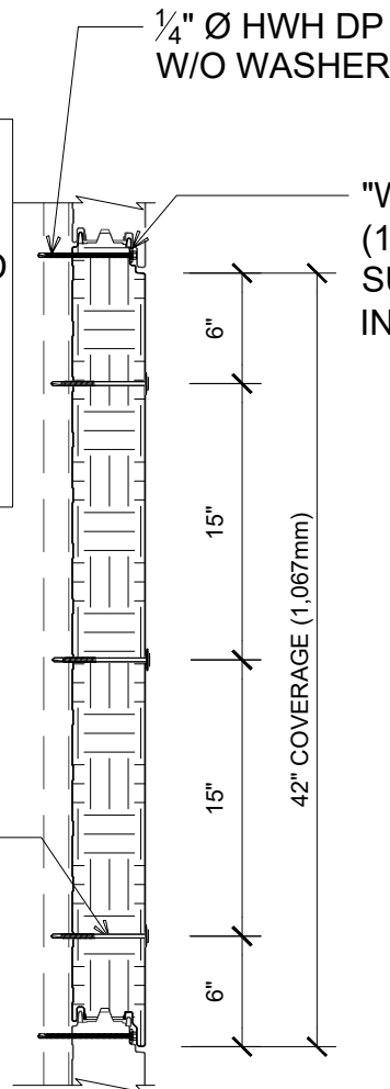
THROUGH FASTENING REQUIREMENTS (3 - THROUGH FASTENER PATTERN EXAMPLE)
