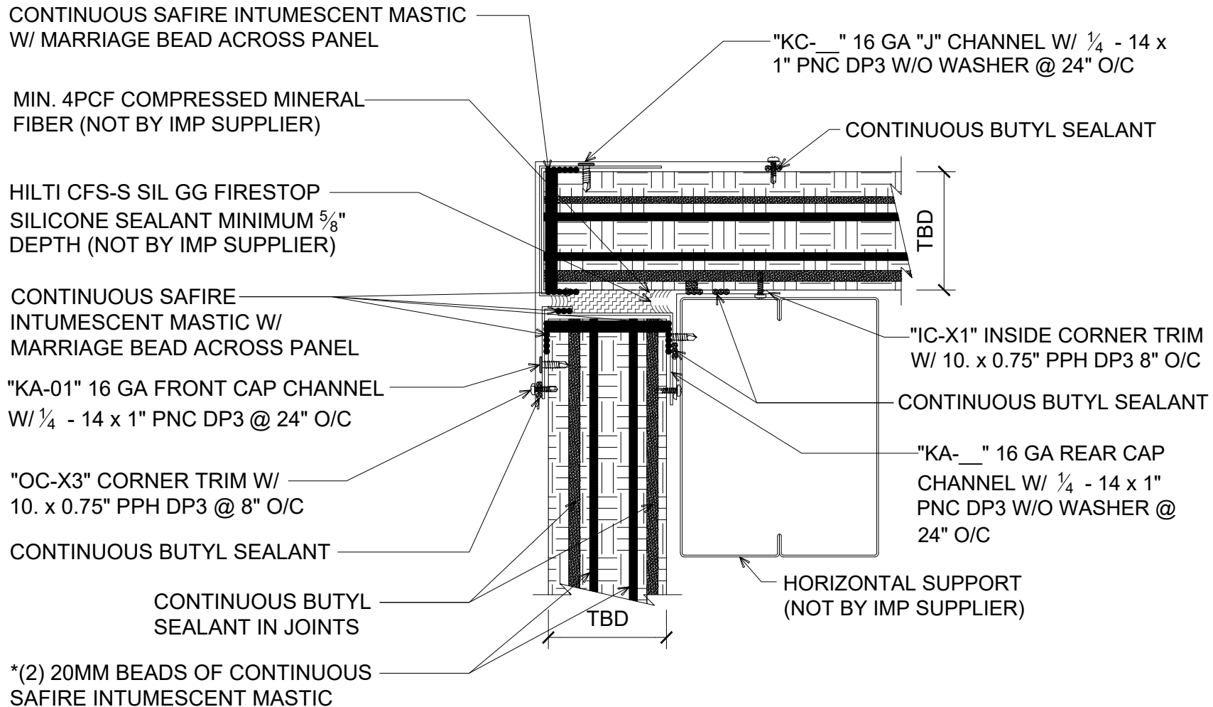
#J OUTSIDE CORNER @ PANEL JOINT FLAT TRIM (4" AND 6" PANEL ONLY) (PLAN VIEW)
